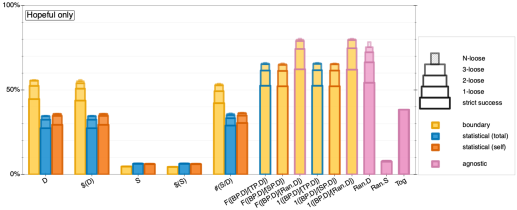
Fig. 3. Average success rates for T = 1 , hopeful only.
